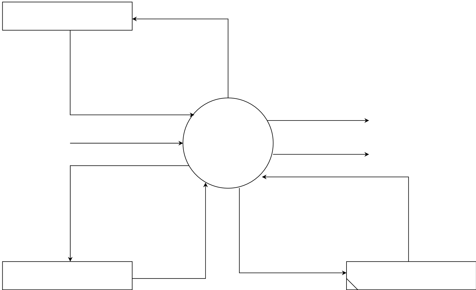
Context Diagram
