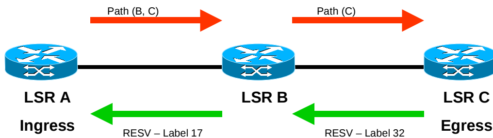
Fig.3 RSVP LSP Setup Flow
