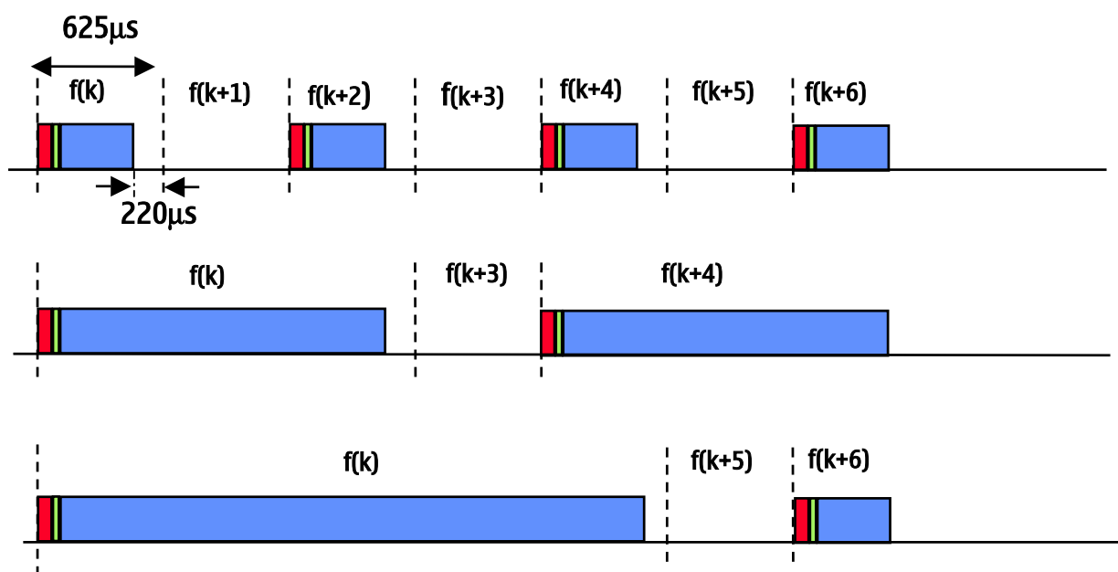
Figure 4. Three-slot and five-slot long packets reduce overhead compared to one-slot packets. 220 \mu s switching time after the packet is needed for changing the frequency.
